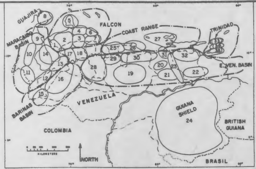
INDEX MAP SHOWING LOCATION OF STRATIGRAPHIC COLUMNS Numbers on map refer to numbers at top of each column
